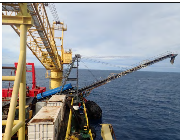
Photo 9. Flyout conveyor where waste materials will go back to the sea
